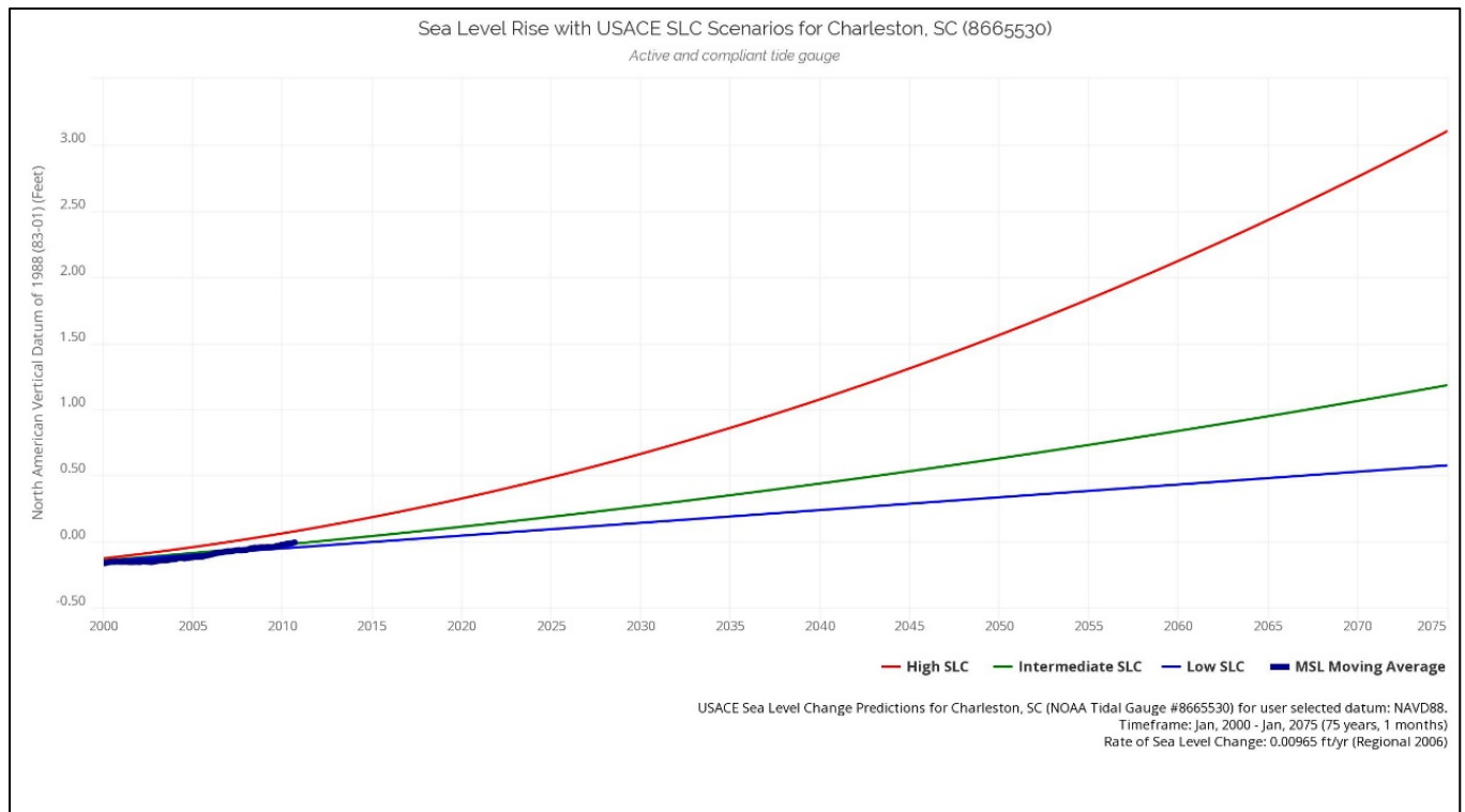
Figure 5-2. USACE Sea-Level Change Scenarios.
