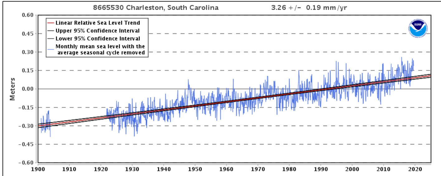
Figure 3-1. Relative Sea-Level Trend, NOAA Gauge 8665530.
