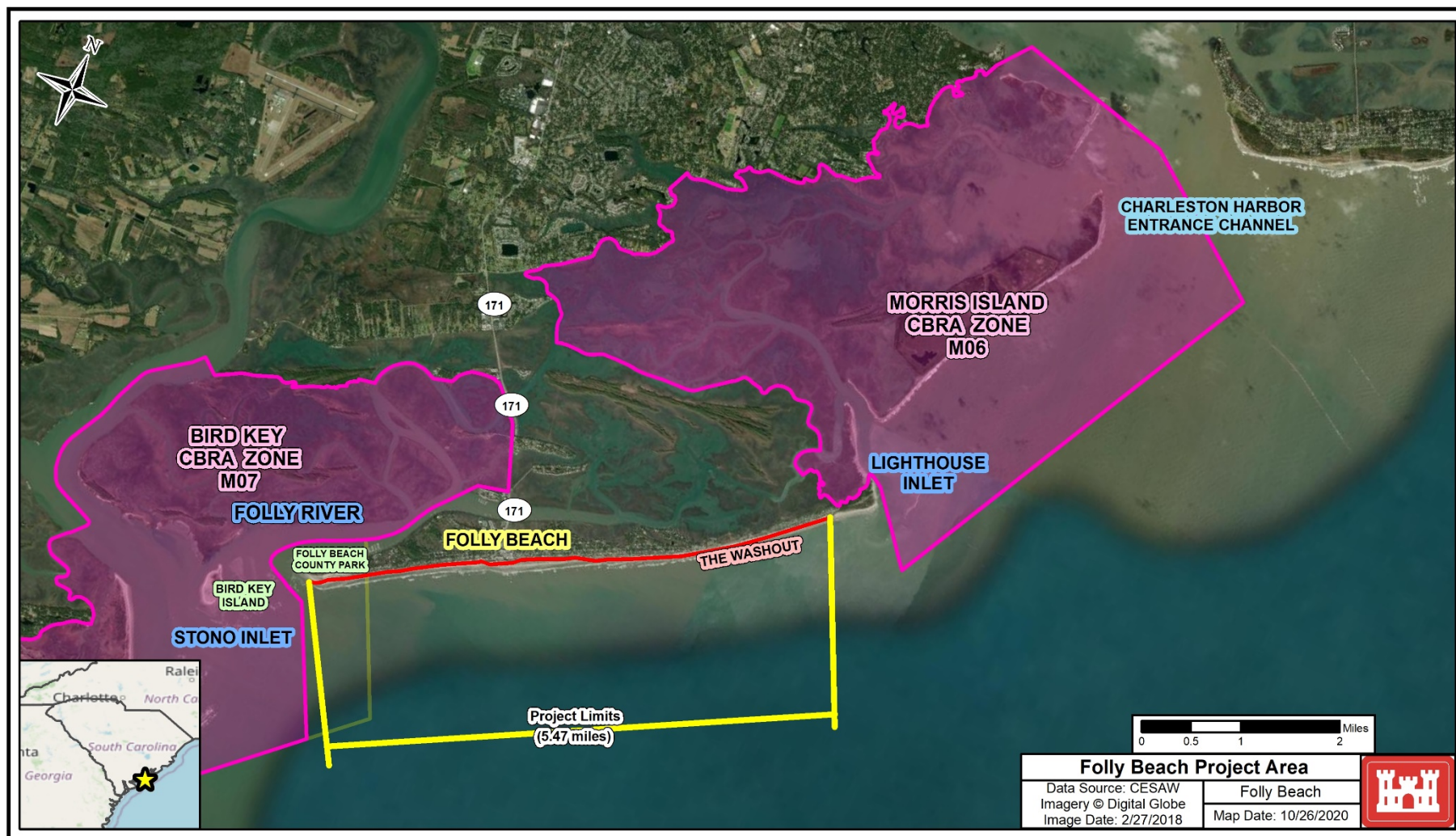
Figure 1-1. The location of the study area in relation to the adjacent Coastal Barrier Resources Act (CBRA) units and Charleston Harbor Entrance Channel.
