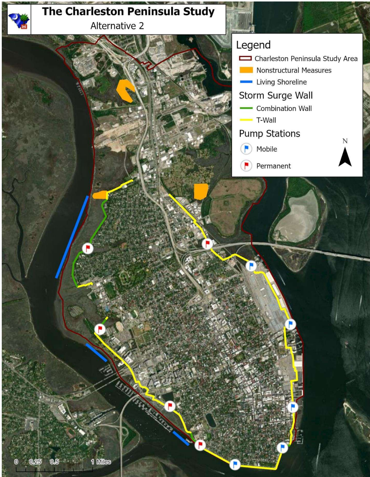
Figure ES-2. The National Economic Development and Recommended Plan. Official mapping product of the Management Support Branch, Charleston District, USACE
