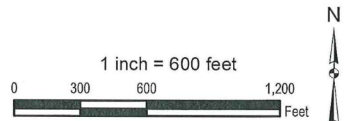
Figure 5: Aquatic Features Map Bull Street Redevelopment Project Richland County, South Carolina Source: USGS Date: July 2015
